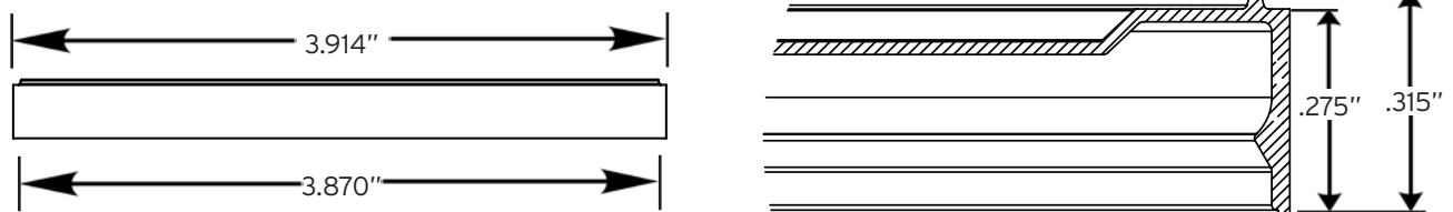
Side View
